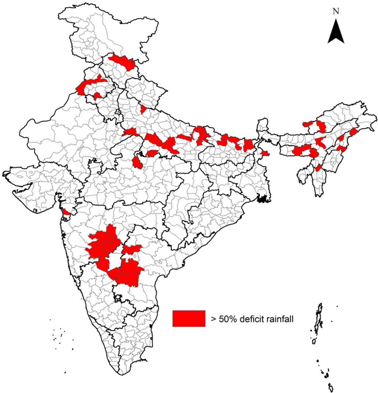
Districts (51) Experiencing more than 50% rainfall deficit (From 1 June – 16 August, 2015)
